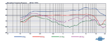
MU-59 Frequency Response
