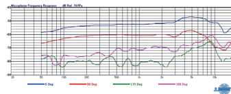
MU-90 Frequency Response
