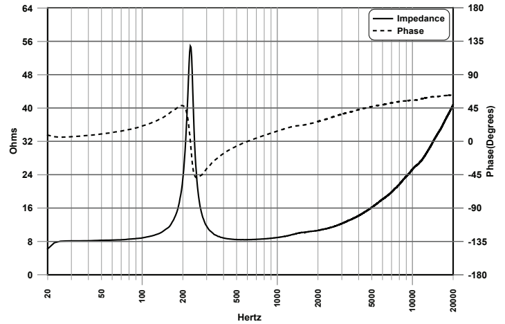
Phase/Impedance Response
