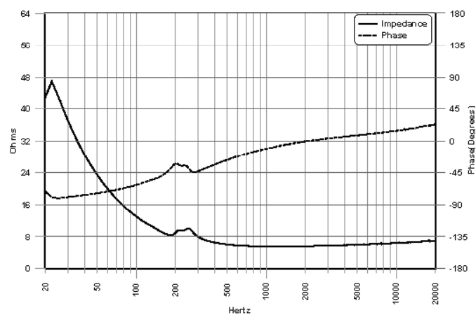
Phase/Impedance Response
